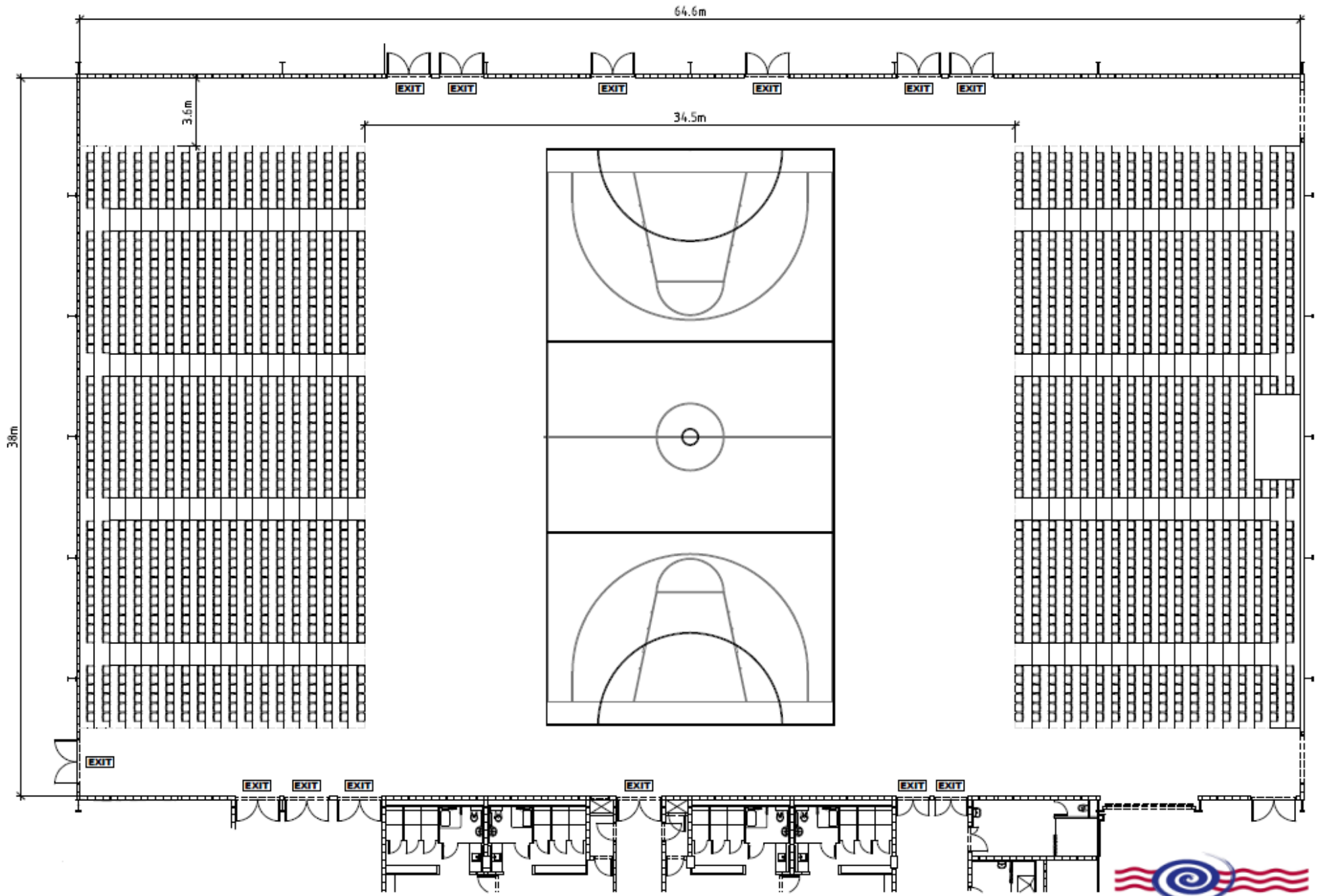
TE RAUPARAHA ARENA MANA COMMUNITY GRANTS FOUNDATION STADIUM RETRACTABLE SEATING LAYOUT
